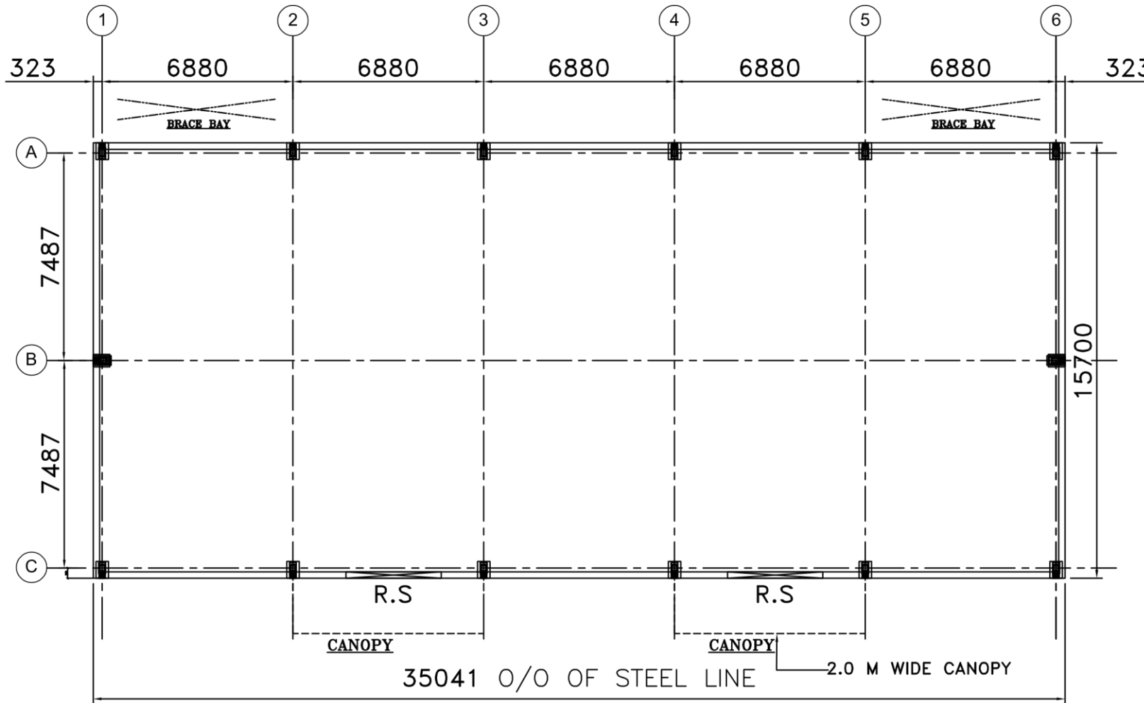
LAYOUT PLAN
